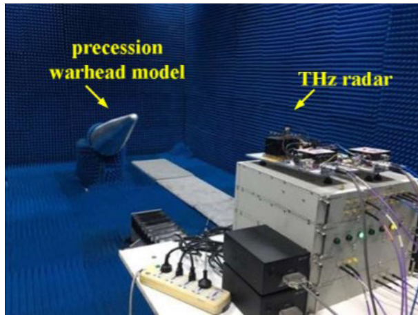
FIGURE 4. THz Radar [13].
