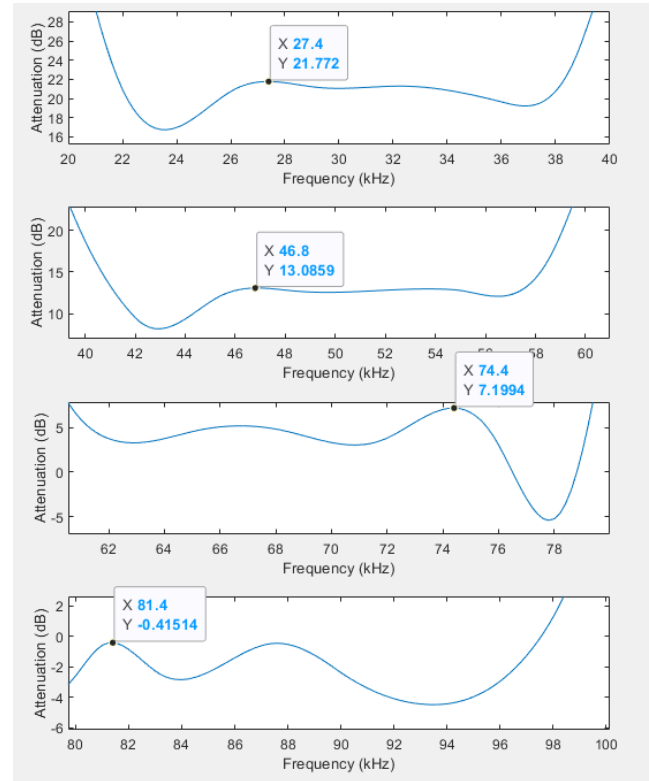
FIGURE 15. The difference between the upper peak envelopes of the spectrums of the first recorded input signal and that at the output after selecting the frames: 20-40, 40-60, 60-80 or 80-100 kHz, consequently from up. Each marker points at the absolute local maximum attenuation of the noise floor, or, in other words, the maximum difference between the envelope of the input and that of the output.
