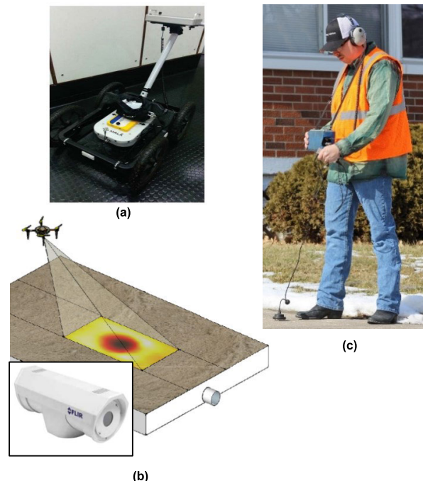
FIGURE 3. Most popular devices that were used in leakage detection: (a) GPR [10]. (b) IR Camera with a model proposing attaching it to a drone [3] (Note that a drone with an integrated IR camera is currently commercially available [11]). (c) Acoustic Detector (An acoustic sensor is placed on the ground and connected to an analyzer held by a worker to process and analyze the received signal and display. The speakers placed on the user's head allow for the listening to ultrasounds converted to audio [12].
