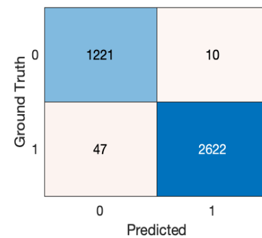
FIGURE 6. Confusion matrices of models "Multi-CNN & HEVC" with Stepwise regression feature space reduction and HEVC-based frame elimination. OVP (top), VSUMM (bottom).
