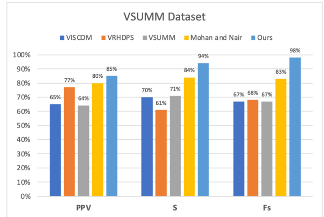
FIGURE 5. This graph shows our top performing model (Multi-CNN & HEVC and HEVC-based frame elimination) in terms of F-score on the VSUMM dataset compared with existing works in the literature.
