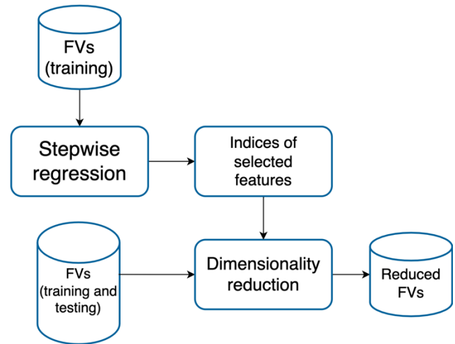
FIGURE 3. General overview of how Stepwise regression is used for feature space dimensionality reduction. SW retains the indices of best features so they can be used later for testing on new data.
