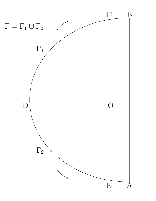
FIGURE 1. The standard Bromwich contour
