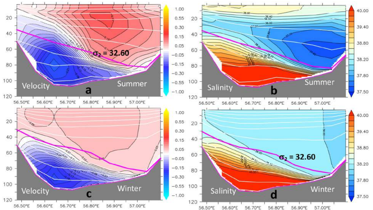
Fig 8. Summer and winter distributions of the meridional velocity and salinity at the Hormuz section (26°N).
