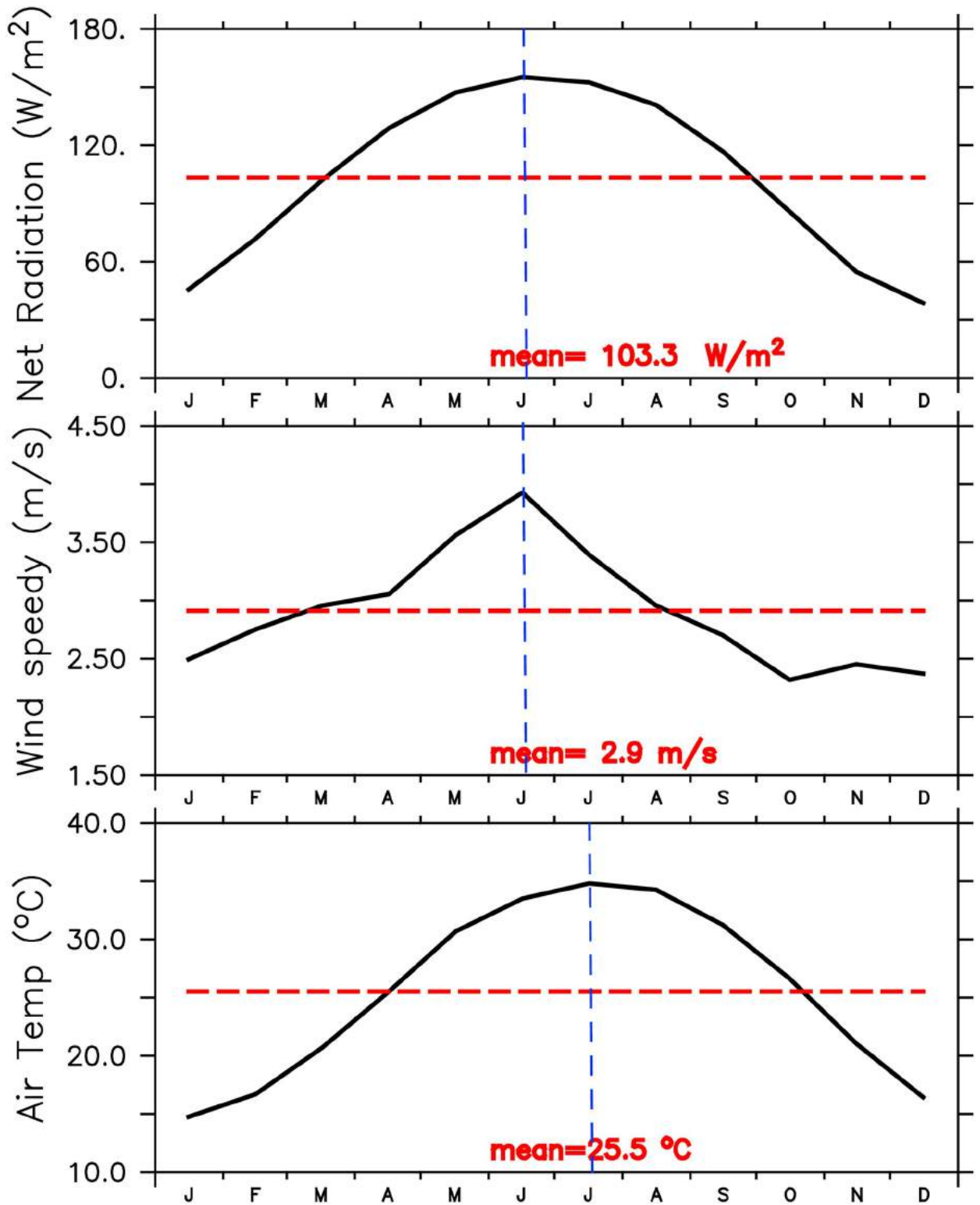
Fig 2. Seasonal variation of the basin-averaged net shortwave radiation, wind speed and air temperature form NCEP.
