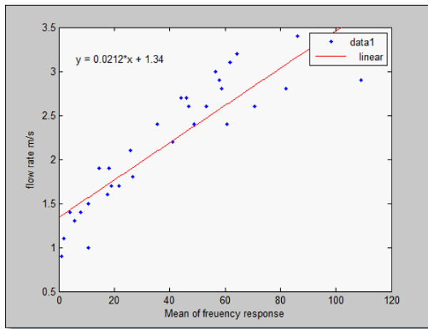
Figure 12: Linear Regression.
