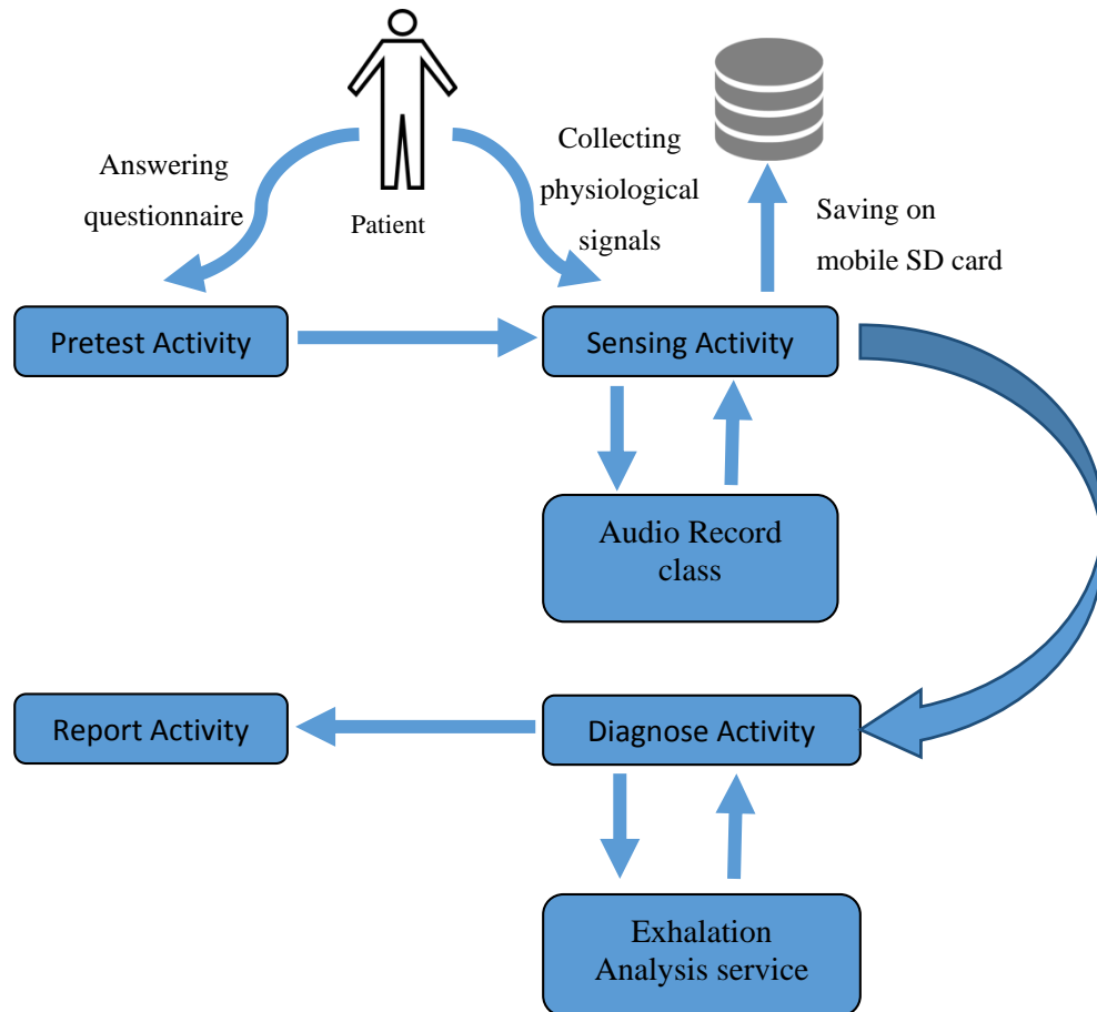
Figure 17: Main activities of the application and their interactions.
