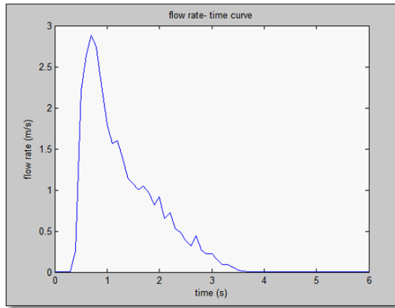
Figure 26: Flow rate vs Time.
