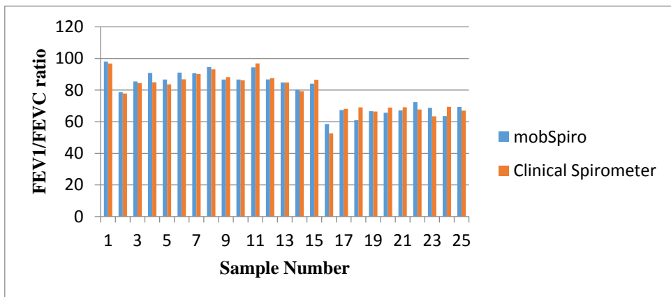
Figure 24: FEV1/FVC ratio differences between real Spirometer result and MobSpiro result.
