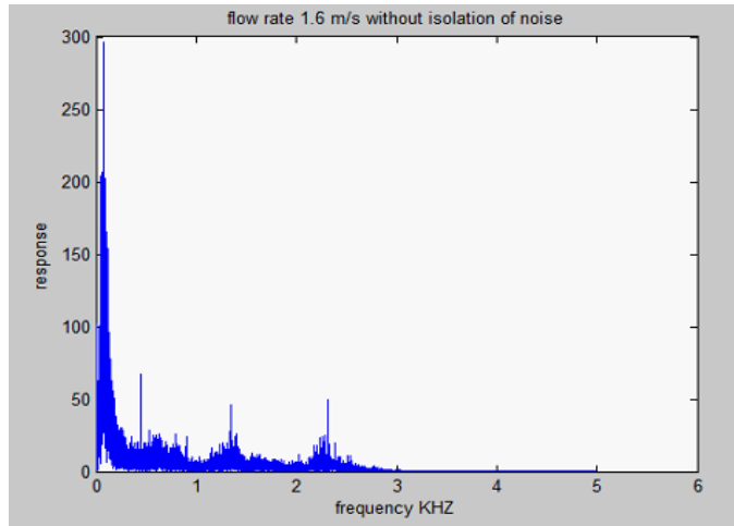
Figure 16: Recorded airflow from non-isolated DYSON fan.
