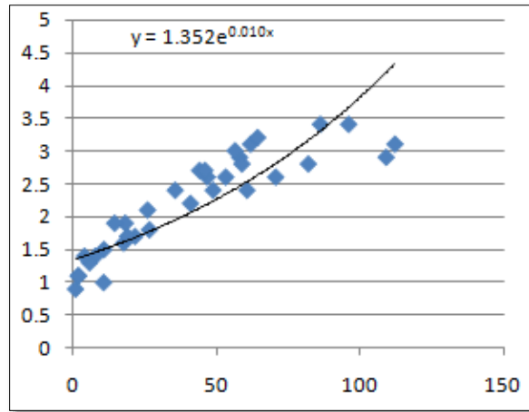
Figure 14: Exponential Regression.
