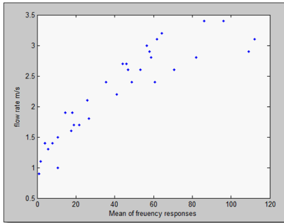
Figure 11: Distribution of data points.
