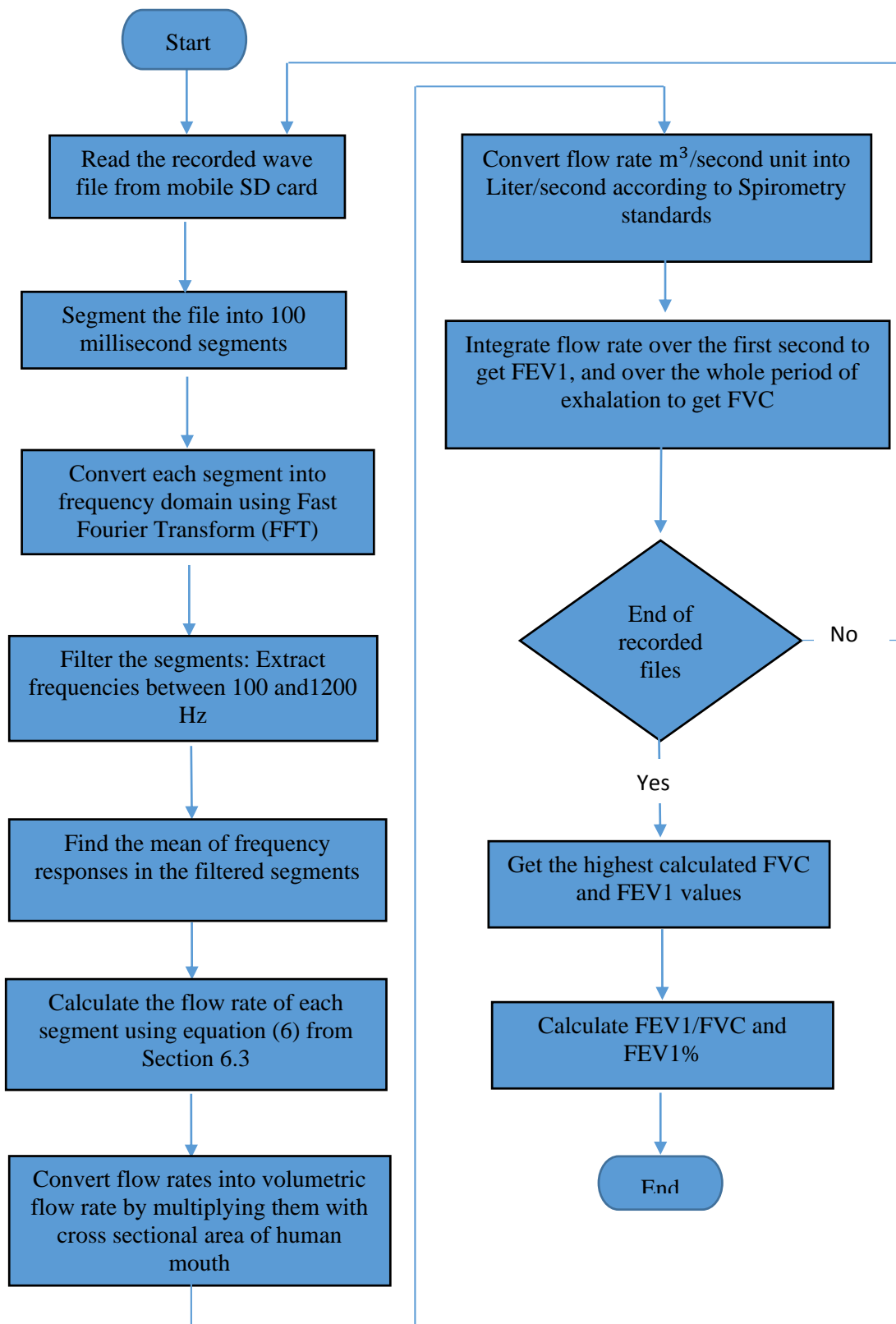
Figure 3: Flow chart explaining how to calculate the parameters FVC and FEV1.
