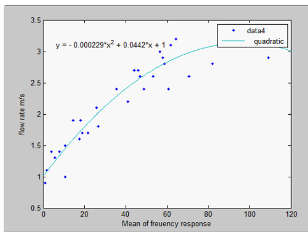
Figure 13: Quadratic Regression.
