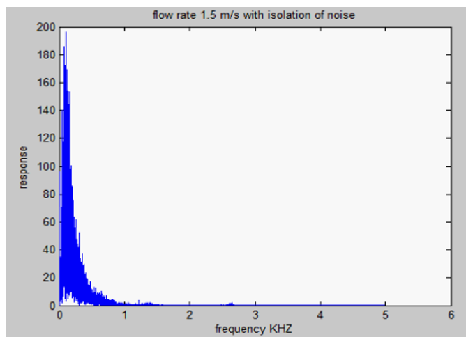
Figure 15: Recorded airflow from isolated DYSON fan.
