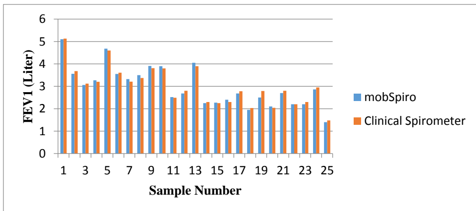
Figure 23: FEV1 differences between real Spirometer result and MobSpiro result.
